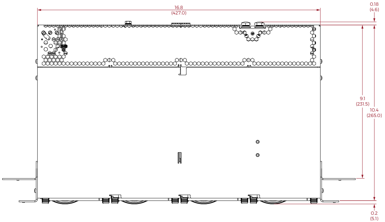
TOP VIEW
