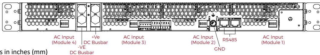
REAR VIEW
