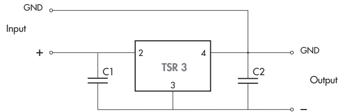
fig. 2 Negative output circuit
