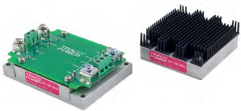
(Models pictured with chassis mount adaptor and optional heatsink)
